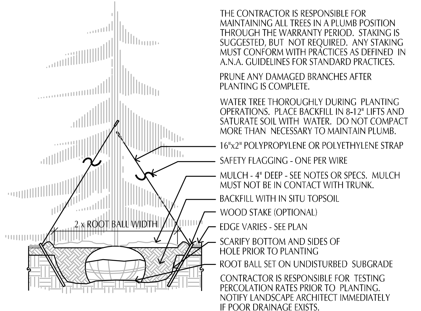
1 L1-1 CONIFEROUS TREE PLANTING DETAIL SCALE: 1/2" = 1'-0"
