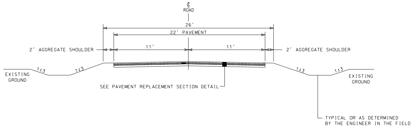
Typical Section
